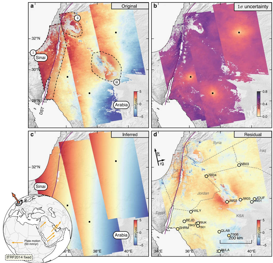
Figure 3. Three overlapping ascending tracks of velocity in northwest Arabia showing the consistent impact of Arabian motion in ITRF2014. (a) Observed line-of-sight (LOS) velocities referenced to the black squares in each of the respective tracks. We masked out areas (i) near and west of the Dead Sea Transform Fault, (ii) a large decorrelated area, and (iii) areas with >100 km wide uplift in Wadi Sirhan Basin. (b) The 1\text{-}\sigma uncertainties of velocities, that is, the diagonals of \mathbf{C}_{d_i}^{0.5} . (c) Inferred Arabian rotation. (d) Arabian-fixed LOS velocities after removing the inferred rotation from (a). Circles: global navigation satellite system horizontal velocities projected into the radar LOS, with the same color coding as Interferometric Synthetic Aperture Radar (InSAR) velocity. Inset globe: the inferred Euler pole from all nine InSAR tracks and the modeled horizontal motions at the five stations used in defining the Arabian Euler vector in ITRF2014 (Altamimi et al., 2017).
