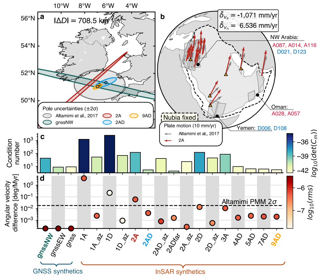
Figure 5. Synthetic scenarios with various sensing geometries. (a) Same style as Figure 4a. |\Delta D| denotes the distance of 2A from Altamimi et al. (2017). (b) Same style as Figure 4d. (c) Model sensitivity: the condition number of \mathbf{G} and the determinant of \mathbf{C}_m . (d) Angular velocity difference from Altamimi et al. (2017) in Cartesian space. Dots are colored by residual RMS. Labeling for global navigation satellite system (GNSS)-only synthetics: gnssNW denotes 15 stations in NW Arabia; gnssEW denotes 20 sparse GNSS sites in panel (b). gnss denotes the full GNSS network in Arabia (Figure 1). Labeling for Interferometric Synthetic Aperture Radar (InSAR) synthetics: the numeric denotes the total number of track(s), “A” denotes ascending data, and “D” for descending data. 1A: one ascending track, A087. 1D: one descending track, D021. 2A: two ascending tracks, A087 and A014. 2ADfar: one ascending in NW Arabia and one descending in Oman, A057 and D021. 2D: D021 and D123. 2AD: A087 and A014. 3A: A087, A014, and A116. 4AD: 3A and D021. 5AD: five tracks in northwest Arabia. 7AD: seven tracks in northwest Arabia and Oman 9AD: all InSAR tracks. The subscript “az” indicates inclusion of the synthetic azimuthal velocity.
