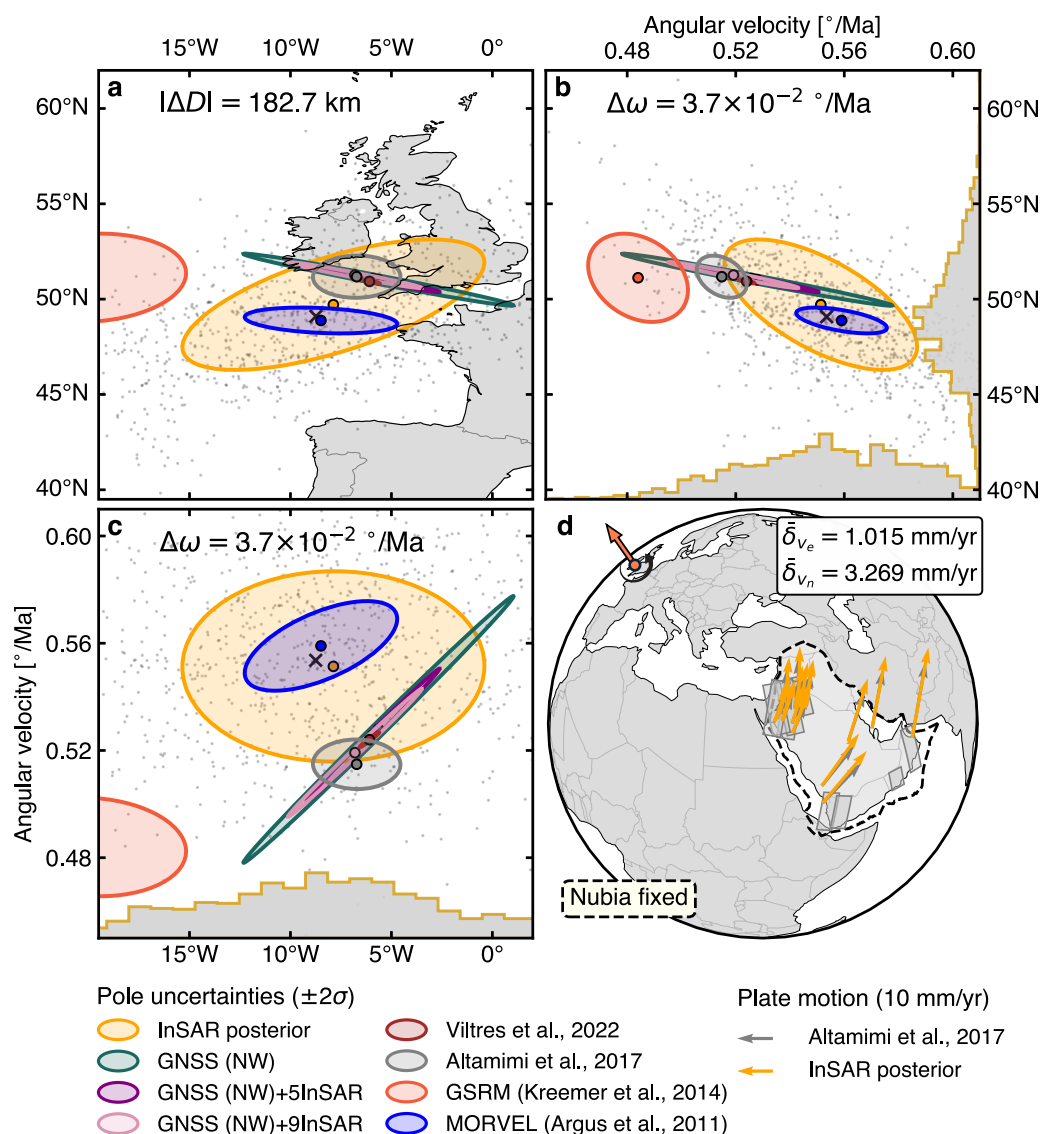
Figure 4. (a–c) Arabian plate Euler vectors (defined in ITRF2014) and uncertainties. The “x” marker shows the vector derived from velocities in Figure 3a. Scattered gray points represent the ensemble of Euler vectors estimated using different reference pixels, with marginal distributions plotted as histograms. The orange ellipse marks the final posterior vector. GNSS (NW) is based on 15 global navigation satellite system (GNSS) stations in northwest Arabia (Viltres et al., 2022), GNSS (NW) +5InSAR is the joint inversion with five Interferometric Synthetic Aperture Radar (InSAR) tracks in NW Arabia, and GNSS(NW) +9InSAR is a joint inversion including all InSAR data sets. |\Delta D| and \Delta\omega are the distance and rotation rate differences between our InSAR-derived vector and Altamimi et al. (2017). (d) Predicted horizontal velocities (in stable Nubia) of the InSAR-only posterior vector evaluated at GNSS sites. The mean differences in east ( \bar{\delta}_{v_e} ) and north ( \bar{\delta}_{v_n} ) components are compared with Altamimi et al. (2017).
