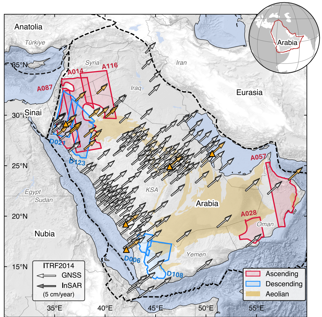
Figure 1. Arabian plate velocities predicted by global navigation satellite system (GNSS)-derived (Viltres et al., 2022, shown as white arrows). The orange arrows are stations used for our geometry tests in Section 3.3. Text S1 in Supporting Information S1 and our Interferometric Synthetic Aperture Radar (InSAR)-derived (dark arrows) Euler vector in International Terrestrial Reference Frame 2014. The orange triangles indicate the GNSS stations used to derive the Arabian Euler vector by Altamimi et al. (2017). Brown shading marks dune regions that decorrelate interferograms. The red (ascending) and blue (descending) rectangles indicate the extent of the InSAR measurements used in this study. Plate boundaries are compiled from Argus et al. (2011), Bird (2003), and Viltres et al. (2022).
